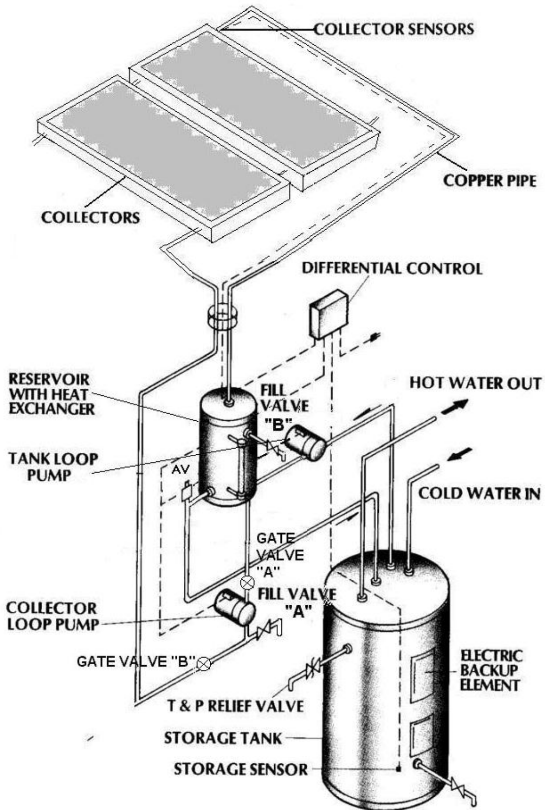
Figure 16. Drainback System with DX Reservoir.
